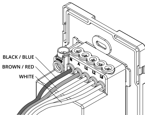
Figure 1: Standard Wiring (Typical L1-L3 wiring, dedicated neutral)
